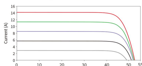
Current-Voltage Curves 595W
